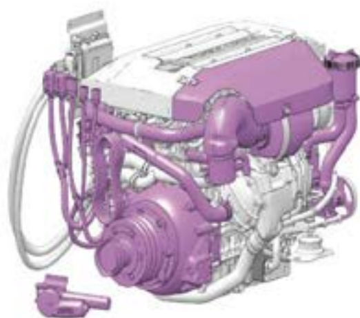
D3 repowering kit. All required components are included, such as adapter ring, exhaust riser, heat shield for turbo and riser, engine cover, installation instructions etc.
